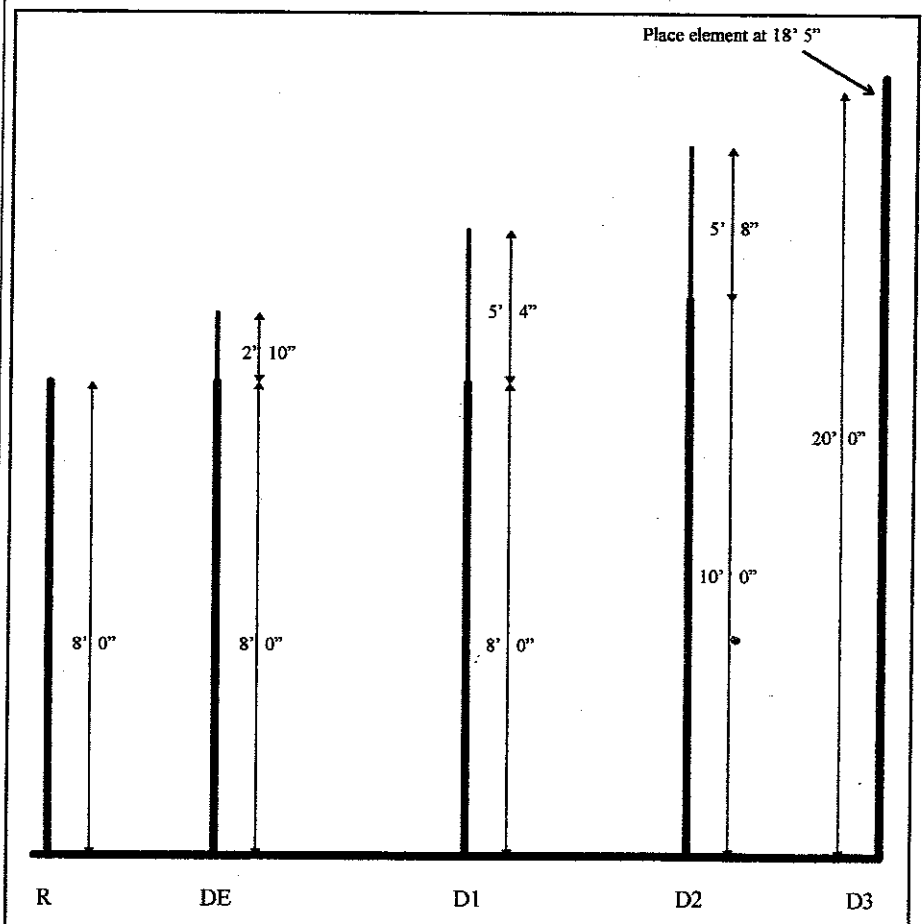
Fig. 4— Physical construction of element supports. The Reflector support is a single 2 × 4 × 8', while the Driven Element and Director #1 are 2 × 4 × 8' topped by a 1 × 2 × 8' cut to the lengths shown. Director #2 is a 2 × 4 × 10' topped by a 1 × 2 × 8' of appropriate length. Director #3 is a 20' length of cyclone rail fencing or two 10' TV antenna masts. The other ends of the elements are tied to eyehooks in the side of the house at the same heights and spacings as the supports.
