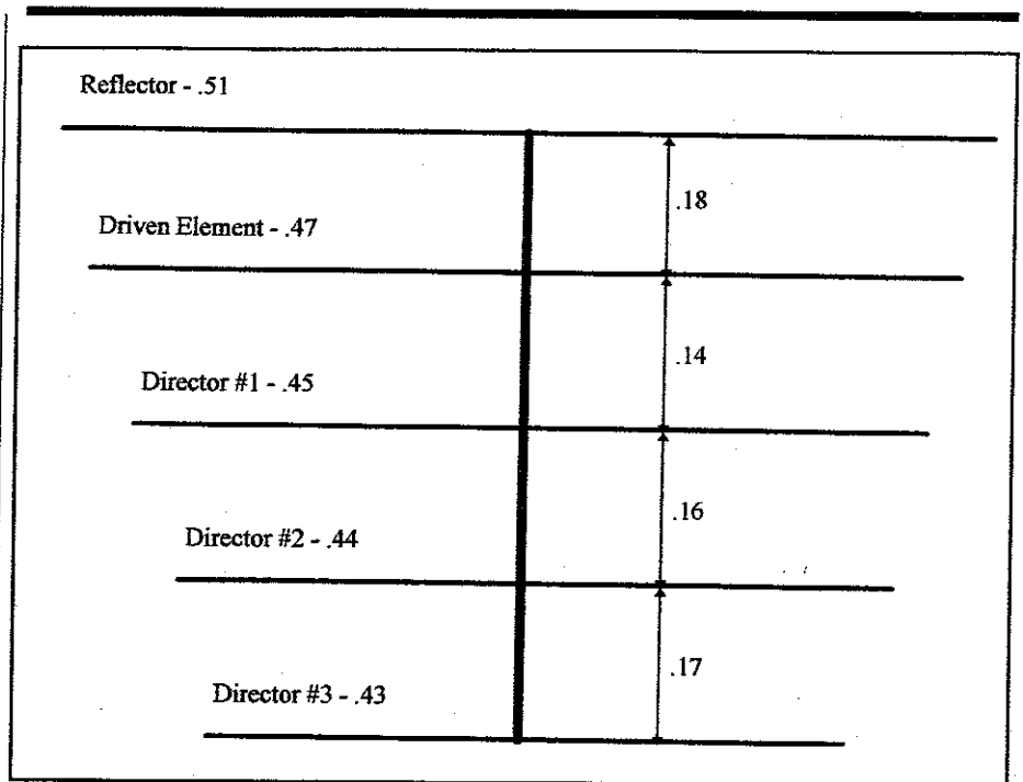
Fig. 3— Top-down view of the Yagi Yagi showing element lengths and spacings in wavelengths. One full wavelength equals 934/design frequency. The elements and boom are not drawn to scale.
