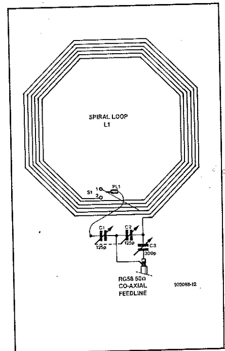
Fig. 2. The QTC Mark 2 circuit.
