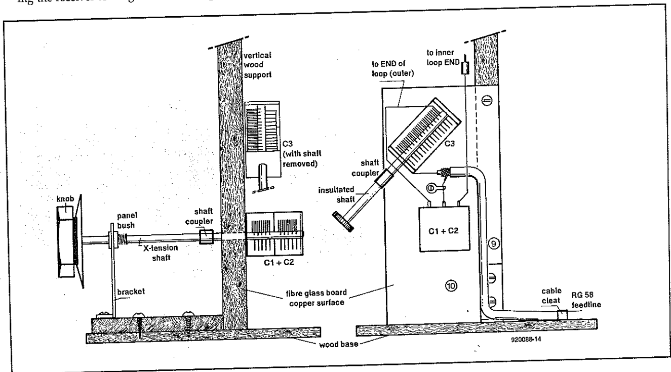
Fig. 4. Panel details.
