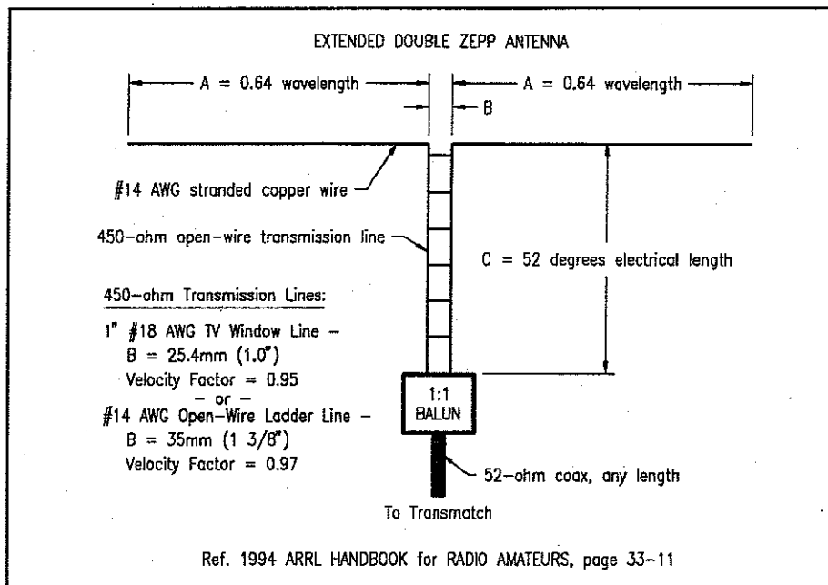
Fig. 1— The extended double Zepp antenna.
