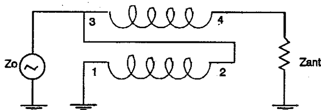
Fig.2: Impedans transformation 4:1
