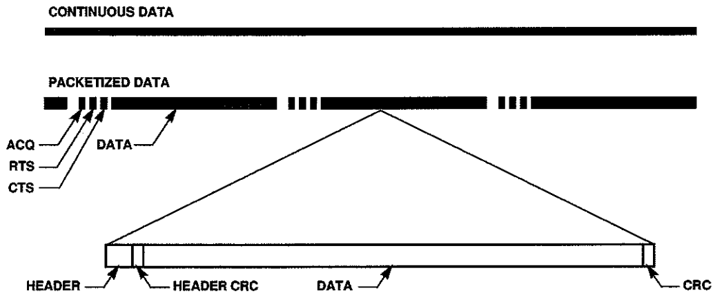
FIGURE 3. PACKET TRANSMISSION
