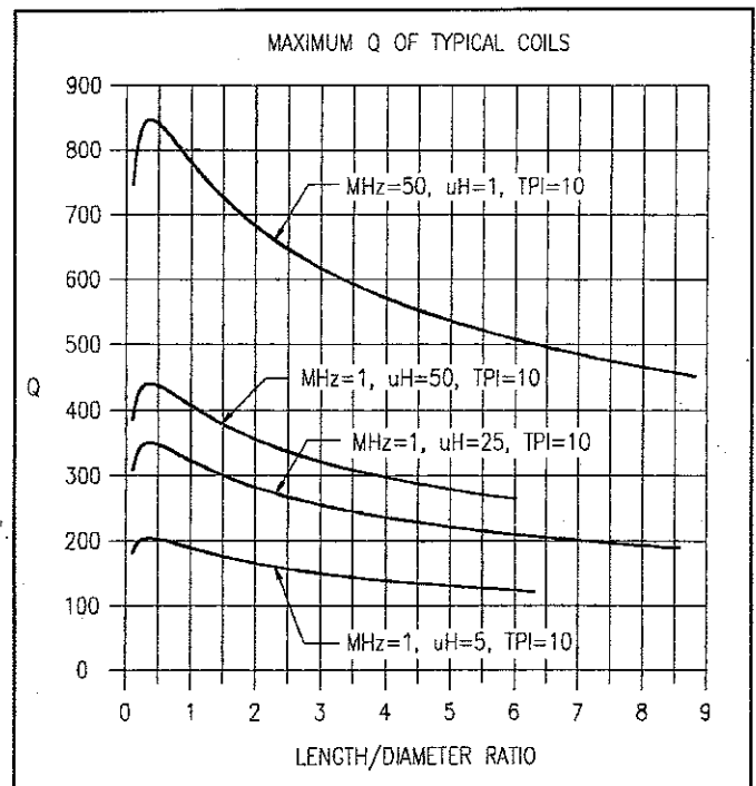
Fig. 5— Maximum Q of typical coils.
