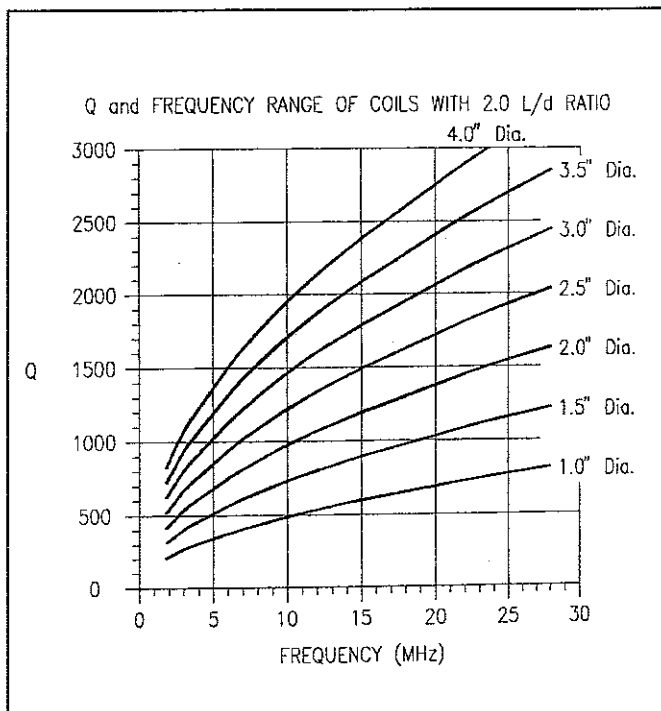
Fig. 4— Q and frequency range of coils with 2.0 L/d ratio.
